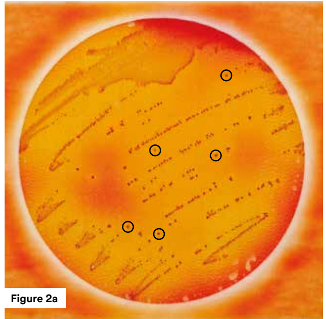
3M Petrifilm Salmonella Express Plate with Presumptive Positive Colonies Circled
